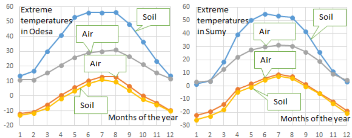
Fig. 3. Average values of monthly maximums and minimums of temperatures
