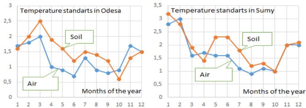
Fig. 2. Standards of the average monthly air and soil surface temperatures
