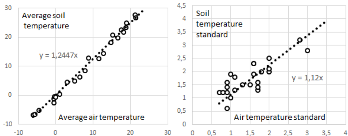
Fig. 4. Dependences between statistical characteristics of the air and soil temperatures
