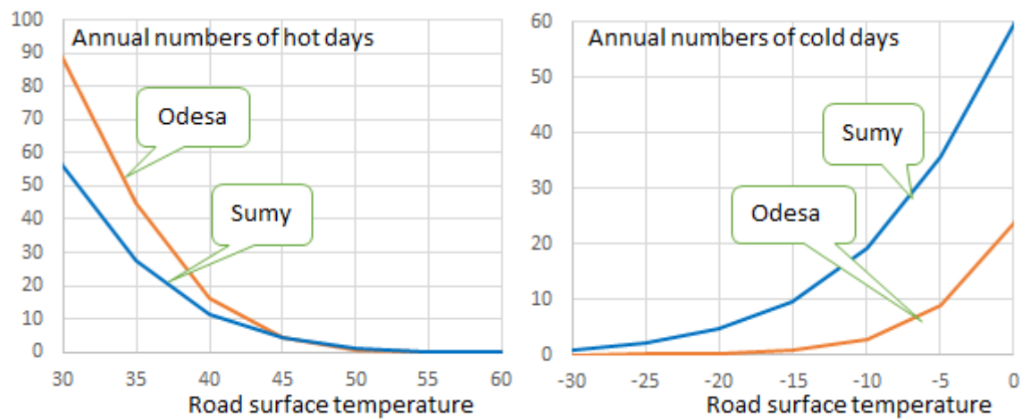
Fig. 9. Annual amounts of hot and cold days corresponding to different values of road surface temperatures X_w and X_c
