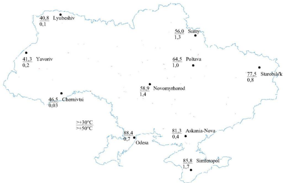
Fig. 12. Annual duration of the hot period
