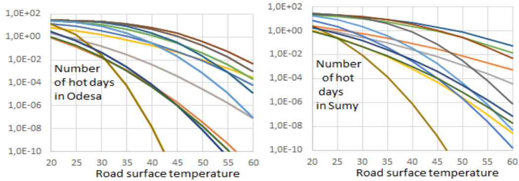
Fig. 7. Monthly amounts of hot days corresponding to different values of the temperature of the road surface X_w
