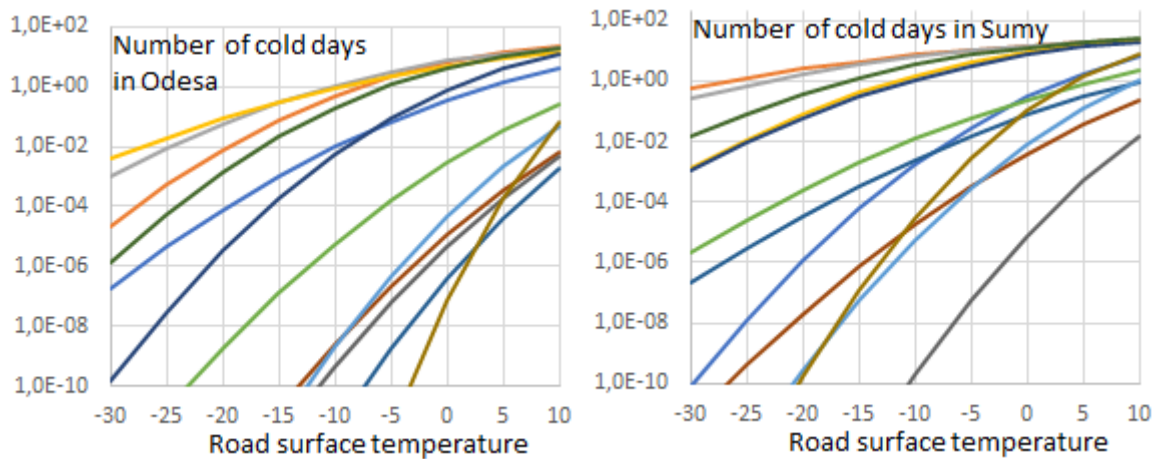
Fig. 8. Monthly numbers of cold days corresponding to different values of the temperature of the road surface X_c
