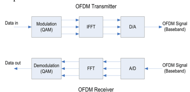
Fig.1. Block Diagram of OFDM Transmitter and Receiver
